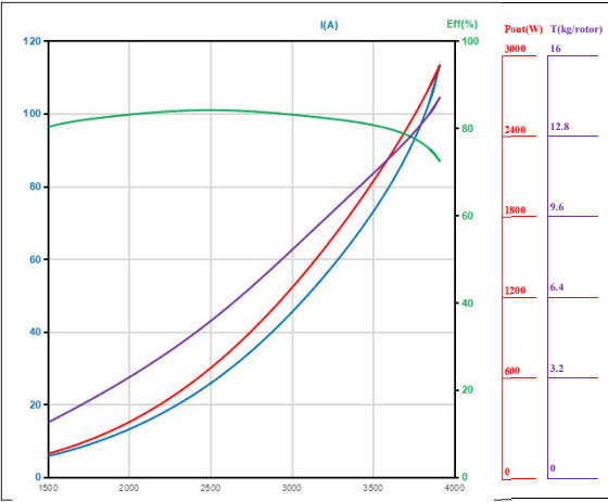
以上数据为室温 25°C、海平面高度的环境下变化油门输入调节拉力测得。 The above data is measured by changing the throttle input to adjust the tension under the environment of 25°C and sea level.
